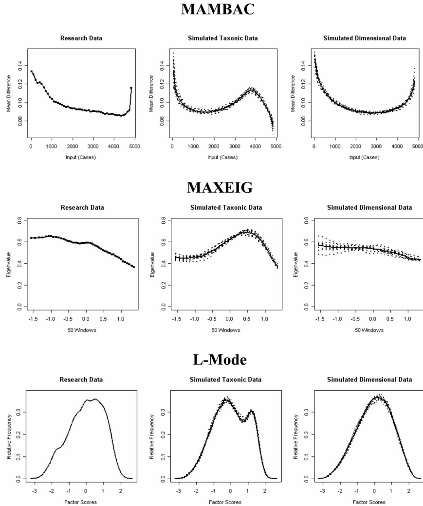
Figure 1. Mean above minus below a cut (MAMBAC), maximum eigenvalue (MAXEIG), and latent mode (L-Mode) results for the summative indicators. Within each three-panel graph, the first panel shows the averaged curve for the research data, and the second and third panels show the averaged curves for the simulated taxonic and dimensional comparison data. For comparison data, each sample's results are represented by a dotted line, with the average across all samples plotted as a solid line.
