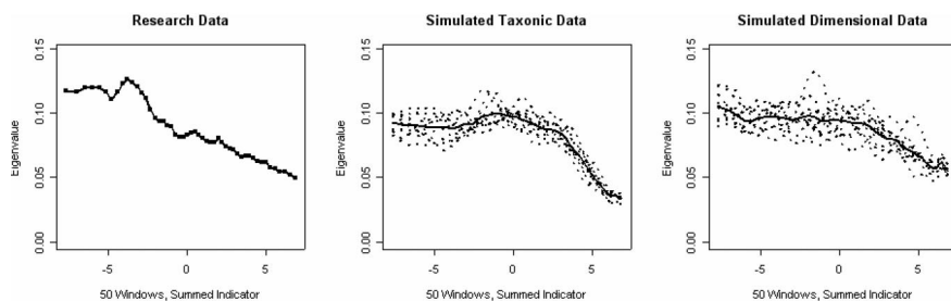
Figure 3. Mean above minus below a cut (MAMBAC) and maximum eigenvalue (MAXEIG) results for indicator sets representing Psychopathy Checklist—Revised (PCL-R) Factors 1 and 2. Within each three-panel graph, the first panel shows the averaged curve for the research data and the second and third panels show the averaged curves for the simulated taxonic and dimensional comparison data. For comparison data, each sample’s results are represented by a dotted line, with the average across all samples plotted as a solid line.
